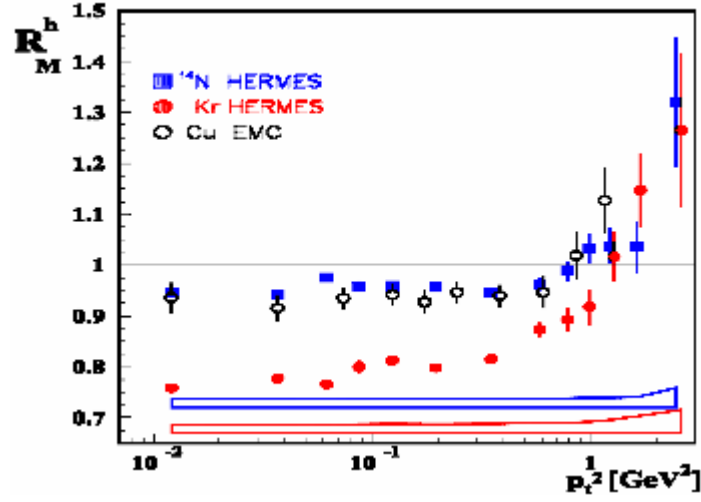
Figure 3. Multiplicity ratio for charged hadrons versus p_t^2 for v > 7 GeV and z > 0.2 . The HERMES data on Kr and ^{14}\text{N} are compared to the EMC [15] data for Cu taken in the range 10 < v < 80 GeV. The error bars represent the statistical uncertainties, while the systematic uncertainty for Kr ( ^{14}\text{N} ) is shown as the lower (upper) band.
