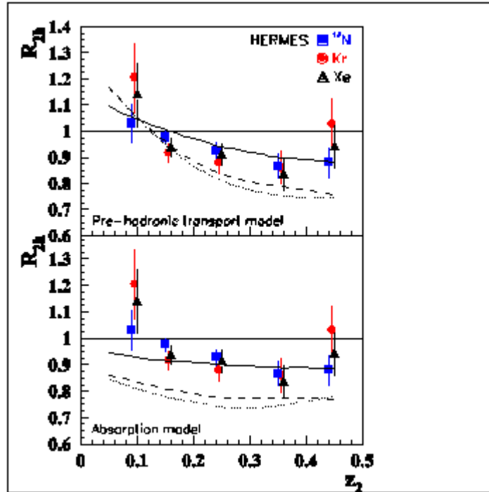
Figure 4. The ratio R_{2h} as a function of z_2 for ^{14}\text{N} (squares), Kr (circles) and Xe (triangles) with z_1 > 0.5 . Only Selection I was considered. The systematical uncertainty is 2% for all the targets and is independent of z_2 . In the upper panel the curves (solid for ^{14}\text{N} , dashed for Kr, dotted for Xe) are calculated within a BUU transport model [4]. In the bottom panel the same data are shown with calculations that assume only absorption for the three nuclei (same line types as in the upper plot) [4].
