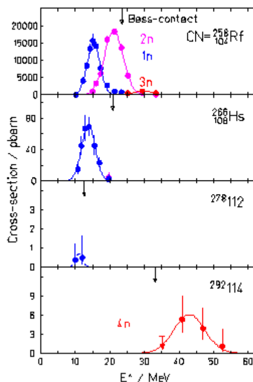
Figure 3. Excitation functions measured at SHIP for the synthesis of elements Rf and Hs plus two data points measured for Z = 112 using cold fusion reactions ( ^{208}\text{Pb} target) [1] and at the DGFRS of FLNR for the synthesis of element Z = 114 [4] using hot fusion reaction ( ^{244}\text{Pu} target). The arrows mark the excitation energy for reactions, when the kinetic energy of the projectile is just sufficient high to reach a contact configuration according to the fusion model by Bass [8]. The excitation energies were calculated using binding energies for the compound nuclei from reference [9].
