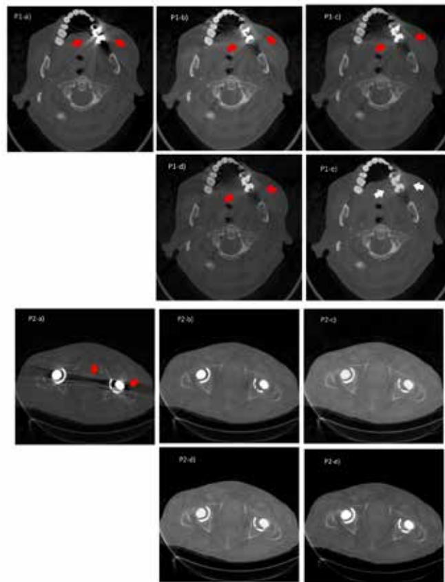
Figure 3. Patient 1 (P1) with two big dental fillings distributed in the right side of the lower jaw and patient 2 (P2) with bilateral hip prosthesis (a) The original artifact CT image (FBP) and the corrected images using the various MAR approaches: (b) LI, (c) NMAR, (d) FSMAR and (e) ISMAR method. The window width and window level was (WW =2500 HU, WL=300 HU).
