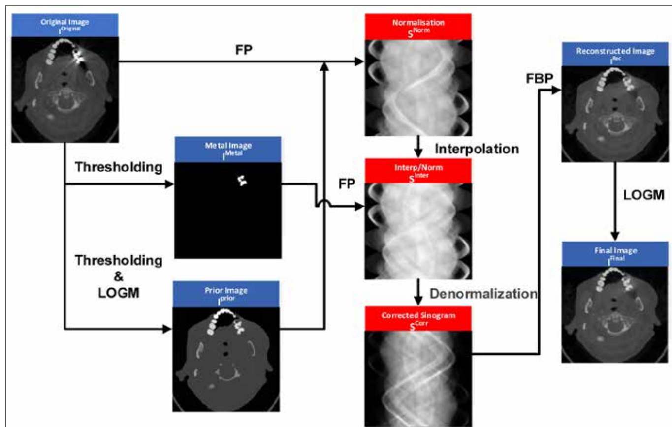
Figure 1. Flow diagram showing the steps of the new MAR based on edge-preserving smoothing via L_0 Gradient Minimization filter algorithm.
