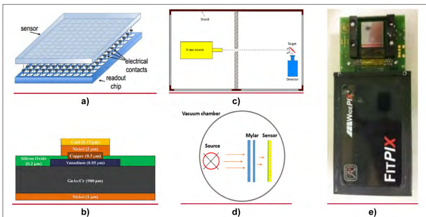
Figure 2.1. a) General scheme of the hybrid detector; b) graphical representation of the single pixel basic structure; c) schematic representation of reflection geometry used for characteristic X-rays measurements; d) schematic representation of the experimental configuration inside of the vacuum chamber; e) hybrid GaAs:Cr Timepix detector with FitPix interface.
