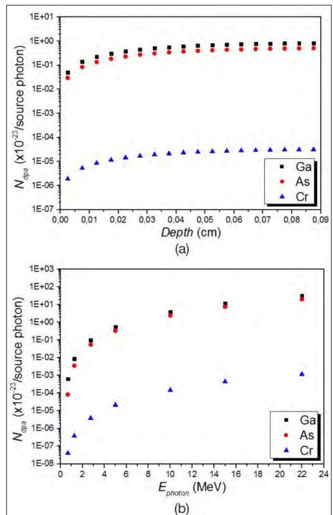
Figure 6. In-depth distribution of the generated dpa number in 900 \mu\text{m} GaAs:Cr irradiated with 5 MeV photons (a), and the behavior of the generated dpa number in GaAs:Cr with the photon energy (b), for each atom species.
