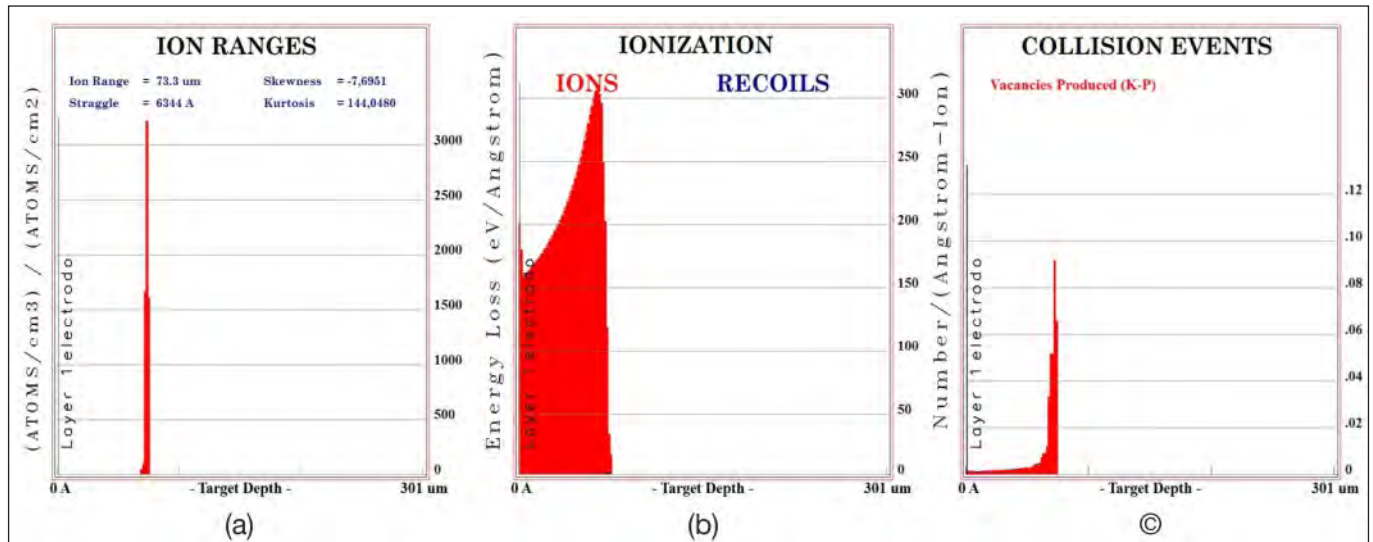
Figure 4. In-depth distributions of stopped ions (a), energy loss (b), and produced vacancies (c), in 300 \mu\text{m} GaAs:Cr for 158.4 MeV ^{22}\text{Ne} ions.
