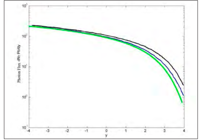
Figure 2. Flux of equivalent photons N_{\gamma/\text{Pb}}(\omega) in p - ^{208}\text{Pb} collision at \sqrt{s_{nn}} = 5.02 TeV.
