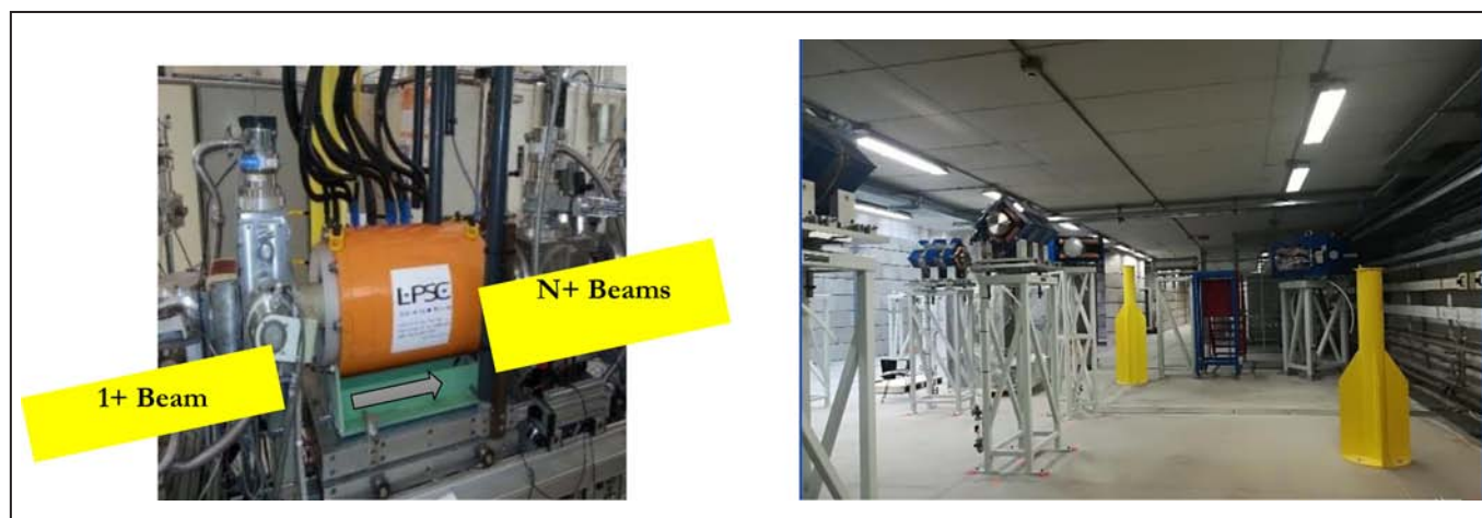
Figure 5. Charge Breeder (left) - Installation of the ADIGE 1^+ line close to the Charge Breeder.
