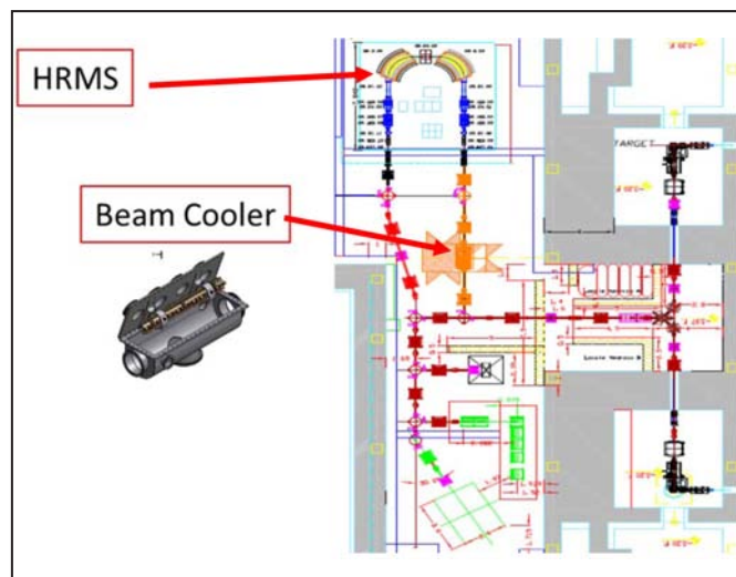
Figure 4. 1^+ Transport Line: from the production bunker to the low Energy Area.
