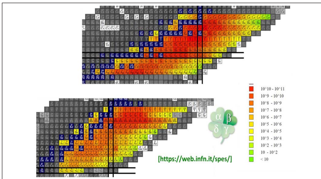
Figure 6. Calculated re-accelerated intensities for SPES: published on the Web site: https://web.infn.it/spes/index.php/news/spes-beam-tables
