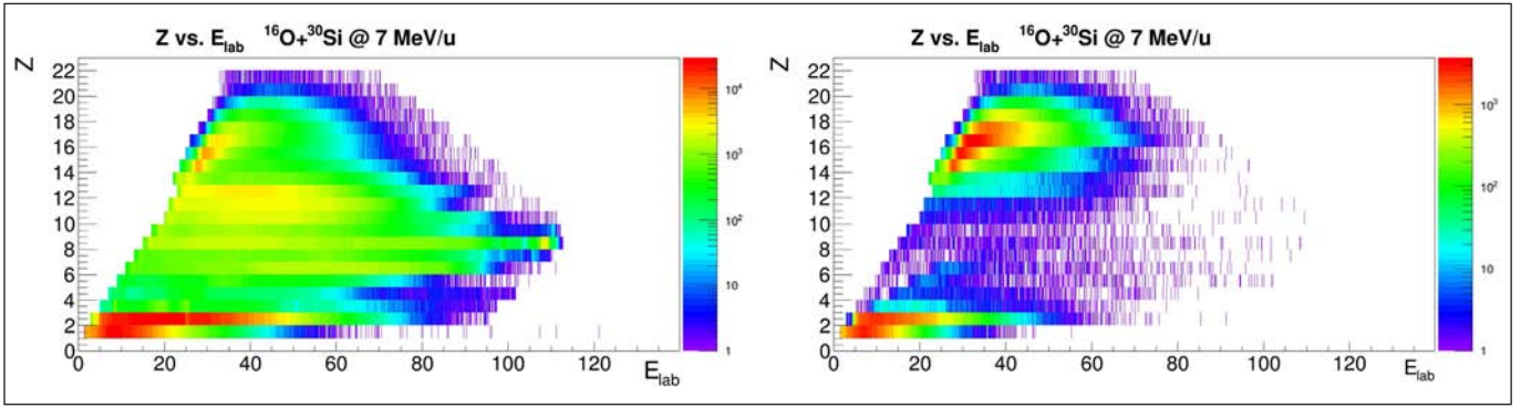
Figure 4. ^{16}\text{O}+^{30}\text{Si} at 111 MeV: Correlation between the detected charge Z and the Energy for total events (left panel) in which the contamination from the reaction on \text{O} is evident (mainly 8 < Z < 13 ) and for selected central events (right panel) with the constrain on Z_{\text{tot}}/Z + Z_{>0.7} and q_i/q_{\text{beam}} < 1.2 (almost complete events).
