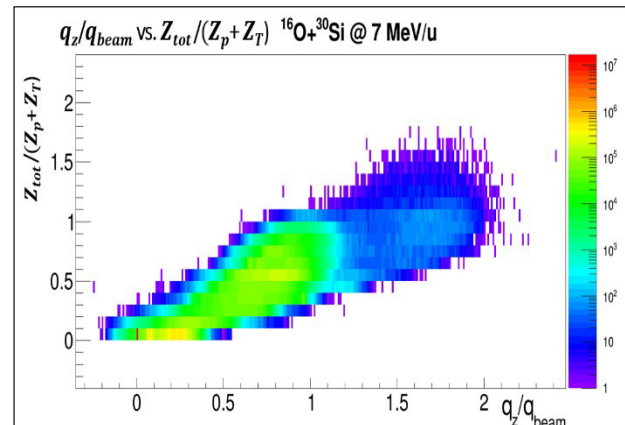
Figure 3. ^{16}\text{O}+^{30}\text{Si} at 111 MeV: distribution of the total detected charge versus the total detected longitudinal momentum. Selections on Z_{\text{tot}}/(Z_p+Z_t)>16 and 0.5<q_z/q_{\text{beam}}<1.2 have been performed to avoid target contamination and random coincidences.
