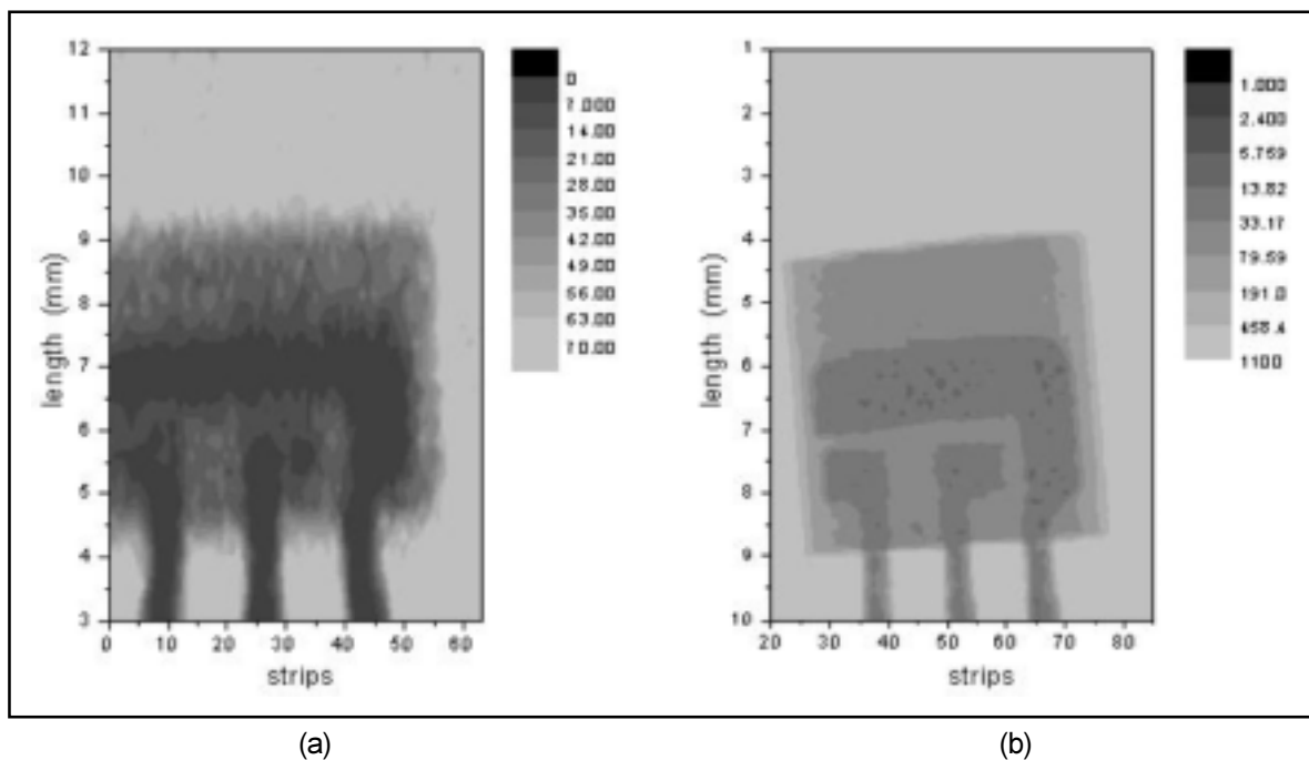
Figure 7. Images of the BC547 transistor at ^{109}\text{Cd} energy using detector front configuration (a), and at 8.04 keV using detector edge-on configuration (b).
