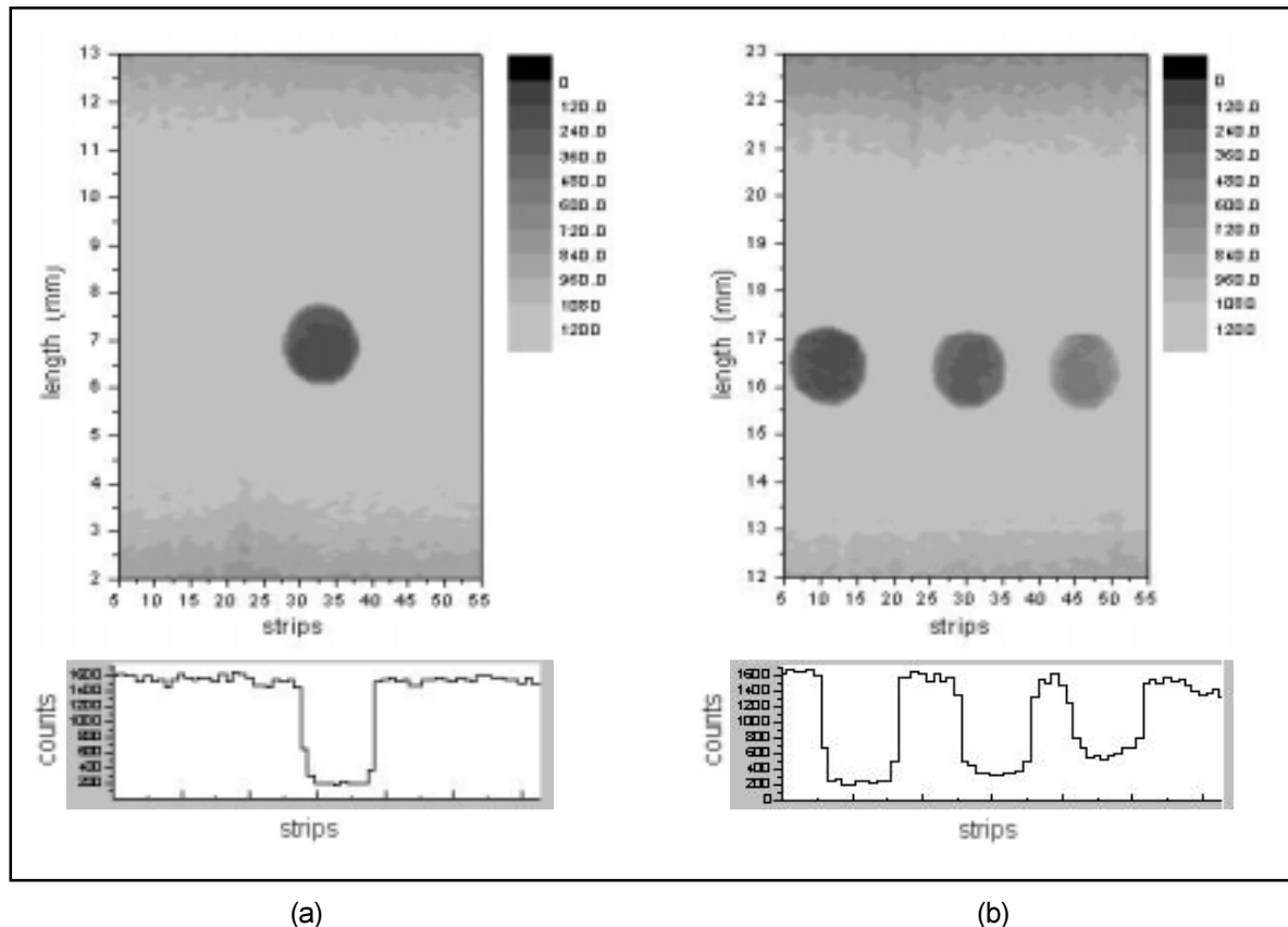
Figure 10. Images and profiles of mammographic phantoms with one microcalcification (a) and with three microcalcifications (b) at 8.04 keV and front configuration.
